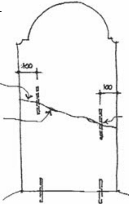
TYPICAL TABLET REPAIR DETAIL
